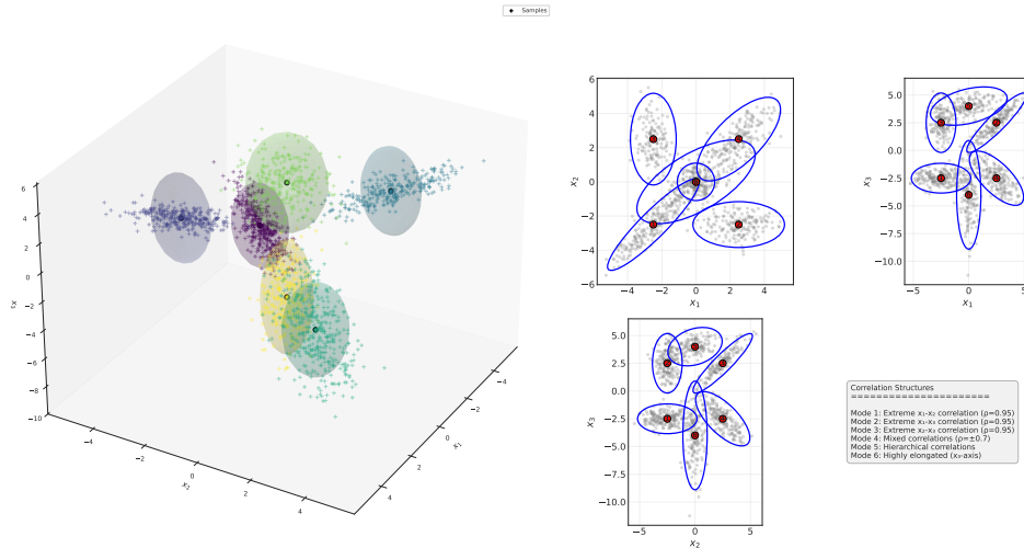
Figure 8: Three-dimensional Gaussian Mixture Model test distribution with complex correlation structures. Left: 3D visualization showing six modes with distinct correlation patterns, where ellipsoids represent 95% confidence regions and colors indicate component membership. Mode 6's extreme elongation along the Z-axis and the planar correlations of Modes 1-3 are clearly visible. Right: Three 2D projections onto coordinate planes (XY, XZ, YZ) reveal the correlation patterns with a summary of correlation structures. The XY projection shows Mode 1's strong correlation; XZ projection highlights Mode 2's correlation; YZ projection displays Mode 3's structure. The correlation matrix for each mode determines the ellipsoid orientation and eccentricity.
