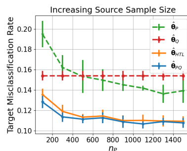
Figure 5: Binary classification results on the CIFAR Dog vs Cat dataset. We use linear classifier with logistic loss. Input features of dimension 512 are extracted by ResNet18. We fix n_Q = 50 and increase n_P . It verifies that our algorithm can work on the general loss.
