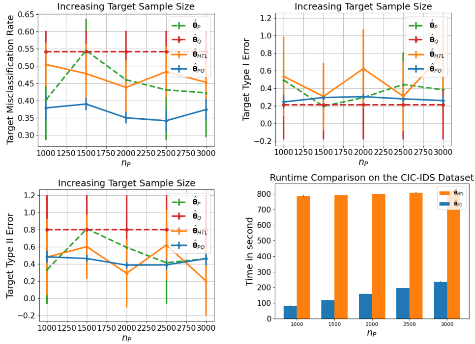
Figure 7: Binary Classification on the CIC-IDS-2017 dataset. We fix n_Q = 1000 (total samples from Q ) and increase n_P (abnormal samples) gradually. (Top-Left) Overall Target Error (Top-Right) Target Type-I Error (Bottom-Left) Target Type-II Error (Bottom-Right) Runtime comparison. Our method ( \hat{\theta}_{PQ} ) achieves better overall accuracy than baselines. We also achieve better and more stable Type-II error than all other baselines. The runtime of our method is also significantly less than HTL.
