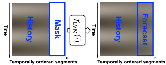
Figure 2: An illustration of an LVM forecaster
