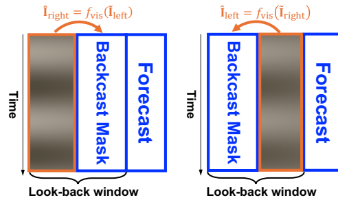
Figure 4: An illustration of BCMASK.
