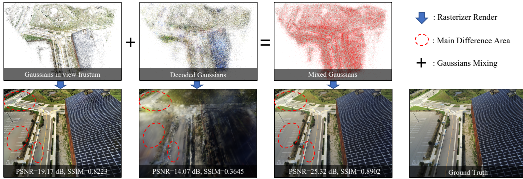
Figure 4. Visualizations of the Gaussians in the view frustum, decoded Gaussians, and mixed Gaussians, along with their corresponding rendered images. It can be observed that rendering with mixed Gaussians leads to better reconstruction of lighting consistency and fine-grained local details.
