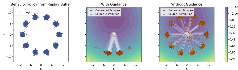
Figure 2: Illustration of Theorem 4.2 on a bandit toy example: (left) behavior data in the replay buffer; (middle) implicit value-guided flow matching steers the policy toward the high-performance behavior policy ( \pi_{\beta^*} ), heatmap shows Q^{\pi_k} - Q^{\pi_{\beta^*}} , white lines indicate transport paths; (right) standard flow matching leads to dispersed sampling with high variance under limited flow steps.
