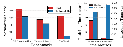
Figure 1: (left) Normalized scores comparing FlowRL and DM-based RL (QVPO) on 12 challenging DMC-hard and HumanoidBench tasks, and 3 DMC-easy & middle tasks. (right) Computational efficiency on the Dogrun task: 1M-step training time and single env step inference time.
