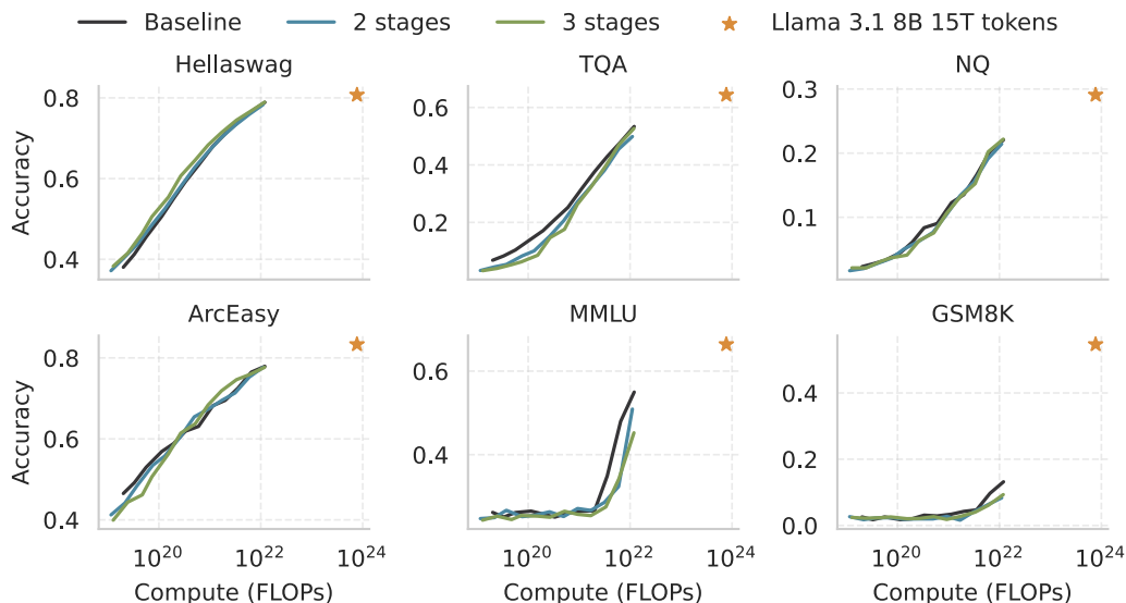
Figure 3: Downstream task performance scaling with compute (1e19-1e22 FLOPs) under data-to-model ratio of 10. AU-Net (2/3 stages) generally tracks a strong BPE Transformer baseline, which itself performs competitively against much larger models (e.g., LLaMa 3.1 8B on 15T tokens 100 \times compute). While AU-Net matches the baseline on tasks like Hellaswag and ARC Easy, and catches up on TQA at higher compute, its performance improvement phase on MMLU and GSM8K appears to start later. The general underperformance on GSM8K is also linked to limited math data in the DCLM pretraining corpus.
