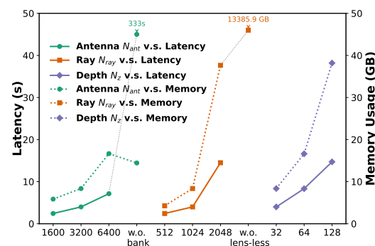
Figure 7: Solid lines indicate latency (time per iteration), while dashed lines show GPU memory usage. Green represents the configuration on patch antenna size in the Signal Tracing Bank. Orange represents the ray number, and “w.o. lens-less” refers to disabling lens-less sampling, whose memory usage is too large to measure experimentally and is instead deduced from theory. Purple represents the number of sample points on each ray.
