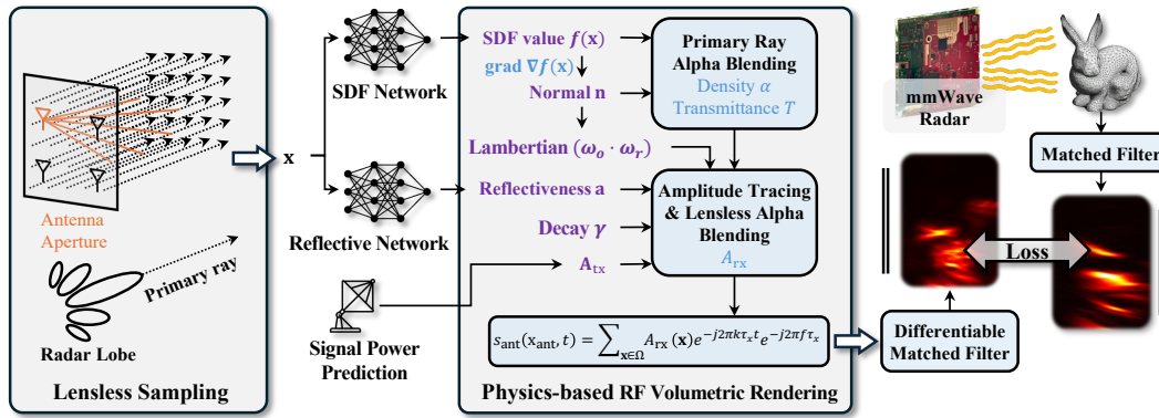
Figure 4: Overview of the GeRaF framework. (1) Lensless sampling replaces ray-based methods. (2) A neural implicit model predicts geometry, reflectivity, and power. (3) RF volumetric rendering simulates physical signal propagation. (4) Matched filtering produces MF power images (heatmaps). (5) An L2 loss compares the rendered and ground truth power for end-to-end training.
