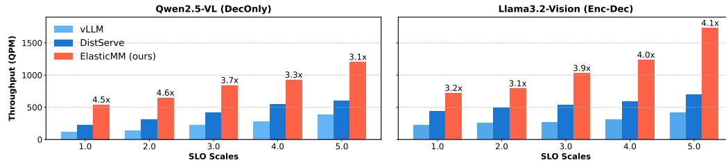
Figure 6: Maximum throughput meeting SLO.
