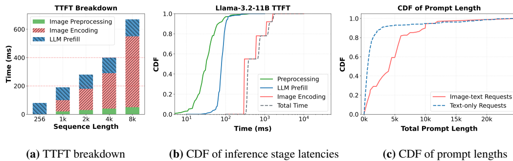
Figure 1: MLLMs' inference overhead and workload complexity. (a) and (b) demonstrate the significant overhead introduced by MLLMs. (c) reveals the longer context in multimodal requests. Results obtained using the LLaMA3.2-11B model on the ShareGPT-4o dataset.
