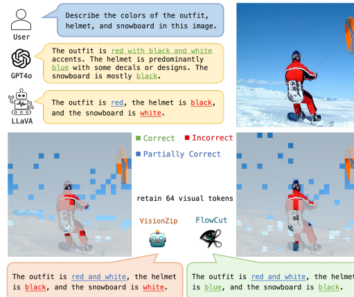
Figure 8: Example comparison of FlowCut and previous SOTA in visual question answering.
