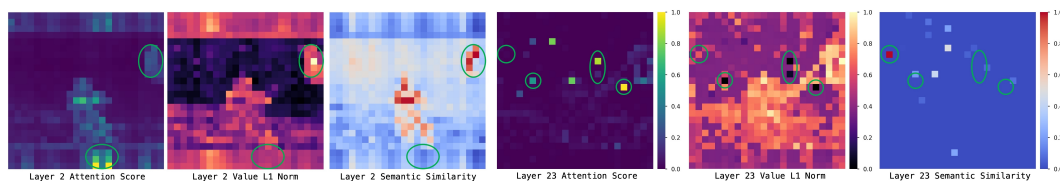
Figure 4: Different criteria for identifying critical tokens can show contradictory results, implying the instability of each single criterion in each single layer.
