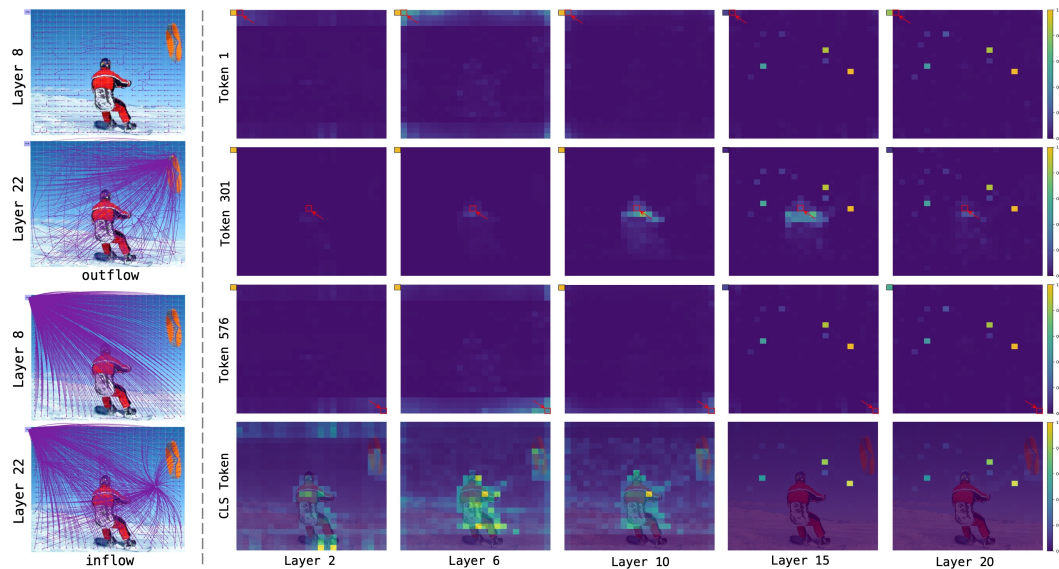
Figure 2: (Left) Information outflow and inflow across vision encoder layers. (Right) Attention map of various tokens across vision encoder layers. Patch tokens engage in sparse, selective information interactions while the CLS token acts as a context relay that gathers and provides information globally.
