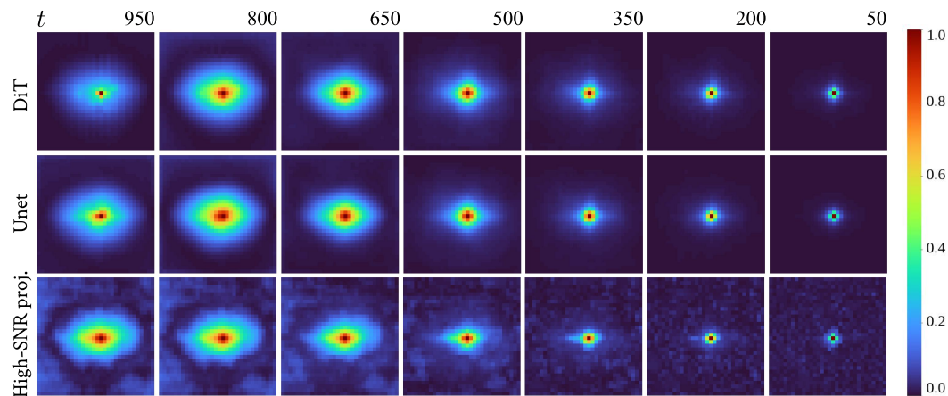
Figure 2: Comparison of sensitivity fields of deep denoisers and the projection operators to high-SNR data's components (i.e. the Wiener filter) on CIFAR-10 dataset. Sensitivity is measured at the center pixel w.r.t. x_0 prediction and throughout a 1000-step DDIM denoising process. Each image is averaged across 32 samples and normalized to [0,1] .
