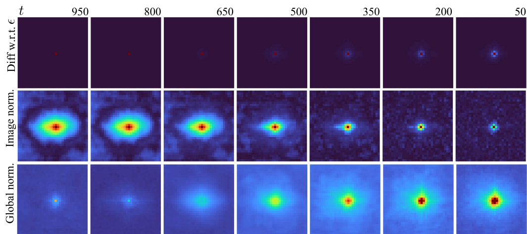
Figure 10: Top: sensitivity field of the noise prediction \partial \epsilon(x, t)/\partial x . Middle: sensitivity field of the image prediction \partial x_0(x, t)/\partial x with per-image normalization. Bottom: the same field with joint normalization across images.
