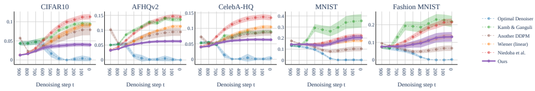
Figure 15: L_2 distance between x_0 prediction and the closest image in the training dataset reported along a 10-step generation trajectory for 5 datasets.
