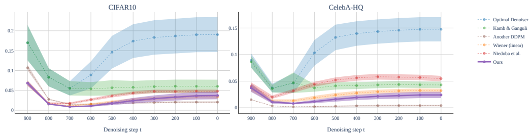
Figure 14: Mean Squared Error (MSE) between the baseline’s predictions and a trained DDPM model. The MSE is calculated on x_0 prediction from each x_t point along a 10-step generation trajectory. The results are presented on the CIFAR10 and CelebA-HQ datasets. Mean and standard deviation values were calculated across 128 samples.
