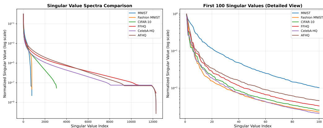
Figure 8: Analysis of the absolute values of the singular values in the covariance matrices across different datasets. Left: across the full set of the singular values. Right: across the first 100 singular values.
