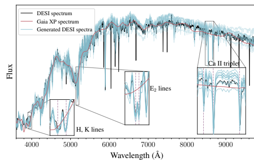
Figure 3: Super-resolution: AION-1 can generate high-resolution posterior spectra samples (blue) conditioned on low-resolution spectra input (red), closely matching the ground-truth high-resolution measurements (black) in line location, width, and amplitude.
