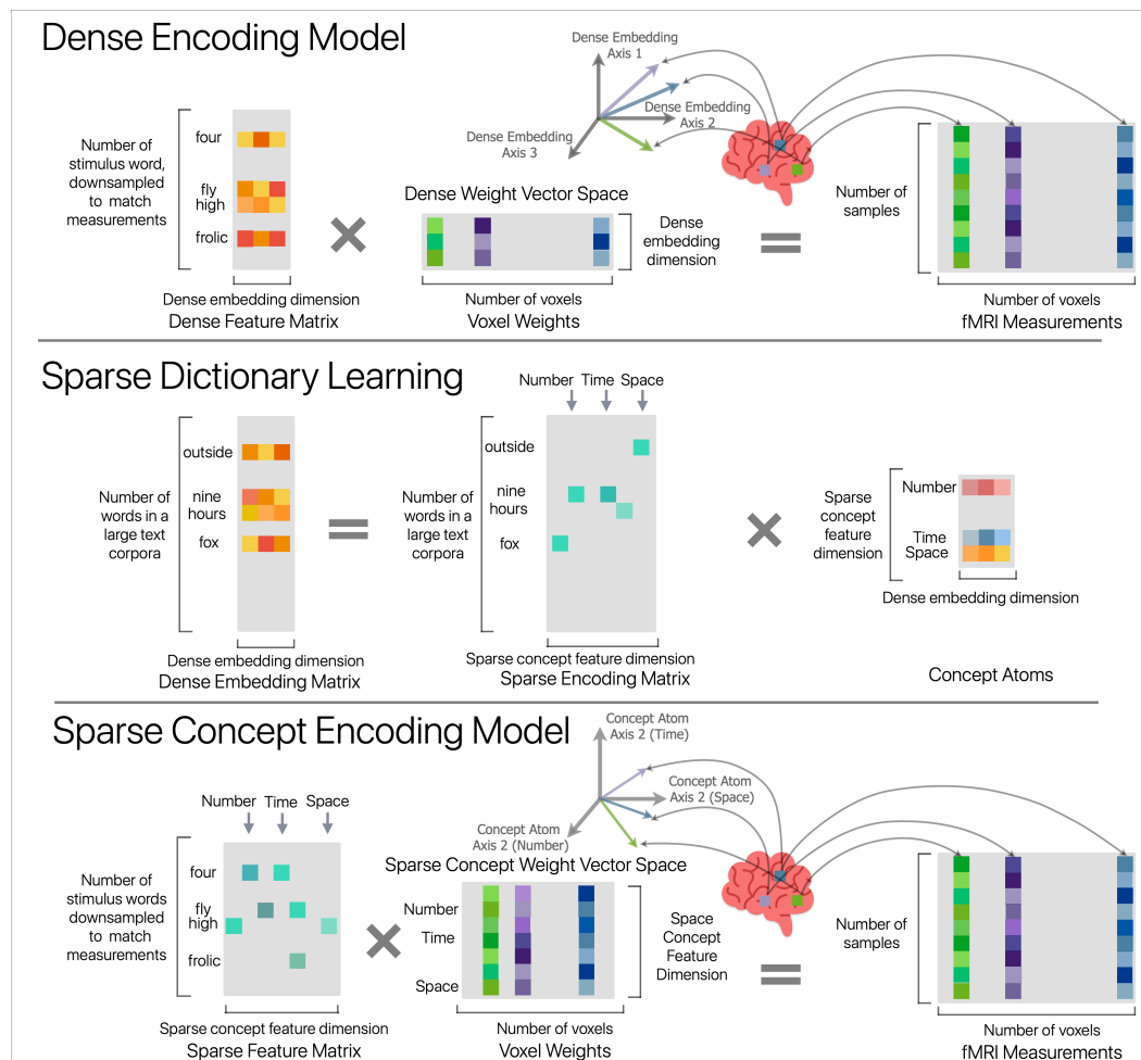
Figure 3: The Sparse Concept Encoding Model produces interpretable voxel weights by replacing dense features with learned concept atoms. Top: Dense Encoding Model: Stimuli are represented using dense word embeddings, resulting in voxel weights that lie in an entangled feature space where semantic directions overlap. Middle: Sparse Dictionary Learning: Dense embeddings are transformed into a higher-dimensional space of sparse concept atoms, each defining a distinct, interpretable semantic axis. Bottom: Sparse Concept Encoding Model: Stimuli are re-encoded as sparse combinations of concept atoms. The resulting voxel weights are defined with respect to disentangled concept-atom axes, enabling direct and interpretable readout of semantic selectivity.
