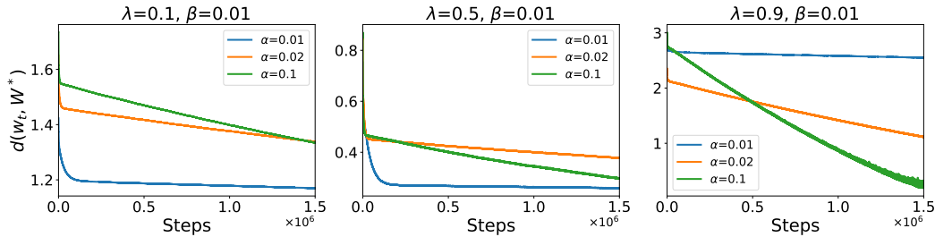
Figure 2: Convergence of (Average Reward TD) with \beta_0 = 0.01, \alpha_0 \in \{0.01, 0.02, 0.1\} . Curves are averaged over 10 runs with shaded regions (too small to be visible) indicating standard errors.
