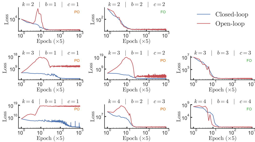
Figure 11: Open- vs closed-loop learning across the k -integrator family. Training loss for closed- (blue) and open-loop (red) RNNs across varying system order ( k ), number of actuators ( b ), and observed variables ( c ). Partial observability (PO, orange) yields sharp loss peaks and occasional non-convergence in open-loop RNNs, while closed-loop RNNs exhibit plateau dynamics before converging. Under full observability (FO, green), both regimes show nearly identical dynamics.
