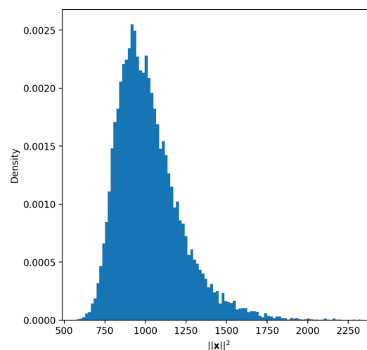
Figure 25: Distribution of \|\mathbf{x}\|^2 on the AFHQ dataset
