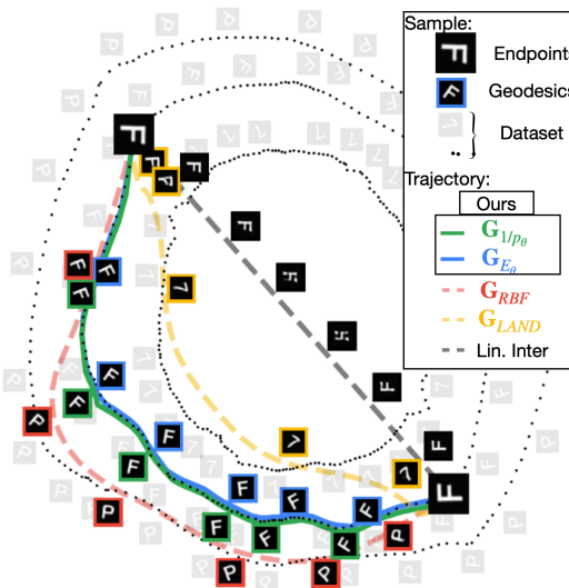
Figure 1: Geodesics visualization for the URC dataset. Trajectories and samples are projected in the PCA space for visualization.
