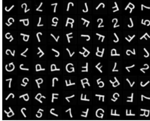
Figure 14: Samples from the EBM train on URC. These samples are generated by applying Langevin dynamics to the energy function learned by the EBM.
