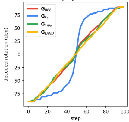
Figure 5: Step size along geodesics in the WCG dataset. Log-based metric ( G_{E_\theta} ) produces sharper variations, reflecting stronger sensitivity to density curvature.
