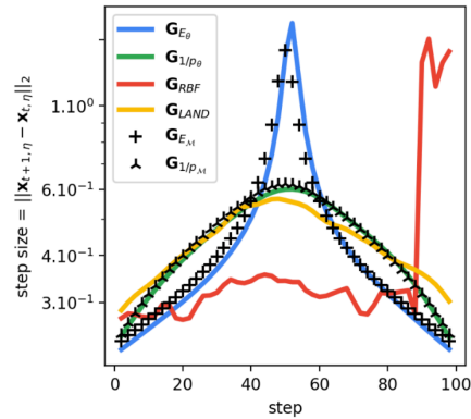
Figure 3: Step size along geodesics in the WCG dataset. Log-based metrics ( G_{E_{\theta}} and G_{E_{\mathcal{M}}} ) produce sharper variations, reflecting stronger sensitivity to density curvature.
