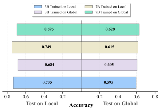
Figure 6: Judge models trained and evaluated on different dataset.
