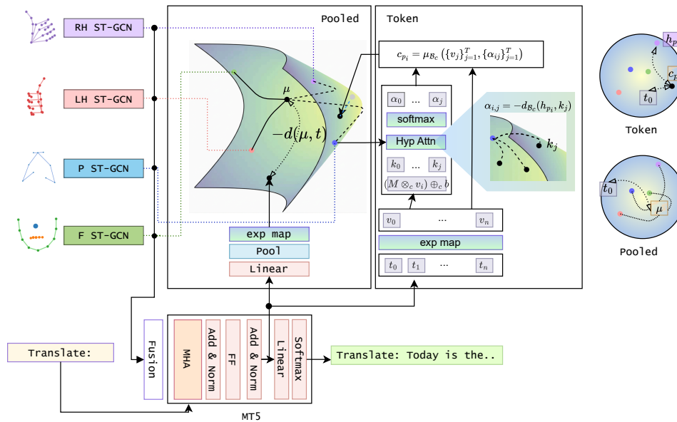
Figure 1: Geo-Sign's hyperbolic framework: (Left) Skeletal features from ST-GCN's for different body parts are projected into a Poincaré ball whose curvature is learned, while the original branch fuses the features for processing via the MT5 language model. (Pooled) The pose features are aggregated via Frechet Mean in Eq.1, while the text embeddings from the final layer of the MT5 model are pooled and projected to the hyperbolic manifold. Geodesic distance between the text embedding and the mean pose features are minimised for positive samples using the contrastive loss in Eq.5. (Token) Alternatively, hyperbolic pose features are used as attention queries against all text embeddings to generate a pose-contextual text embedding. Note the movement of the text features c_{pi} in grey towards the pose feature in blue. (Right) A representation of the Poincaré disk demonstrating the difference between Token, and Pooled methods in the tangent space.
