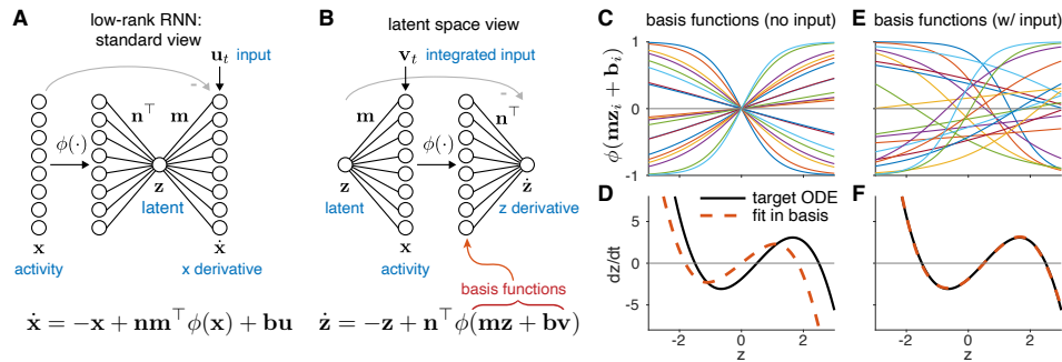
Figure 1: Two equivalent views of low-rank RNNs. (A) Standard view of rank-1 RNN with 8 neurons x and 1 latent dimension z . (B) Alternate view of the same network, now framed in terms of the dynamics of latent z . This shows that a low-rank RNN is equivalent to a neural ODE with a single hidden layer [35]. (C) Basis functions obtained by sampling slope parameters m_i \sim \mathcal{N}(0, 1) , but without input ( v_t = 0 ). (D) Attempting to fit an example ODE using this basis recovers only the odd-symmetric component, since all basis functions are odd symmetric. (E) Adding inputs allows basis functions have random horizontal offsets. Here we sampled the input weights b_i \sim \mathcal{N}(0, 1) and set input v_t = 1 . (Note that this could also be obtained by using per-neuron “biases”). (F) Least squares fitting of n using the basis from (E) provides good fit to the target ODE.
