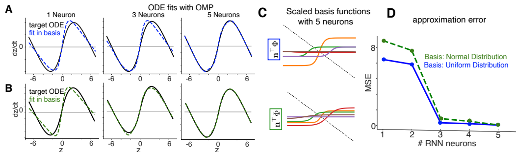
Figure 13: Influence of distribution of basis functions. (A,B) RNN estimated fit of Bi-stable attractor ODE the true underlying ODE over 1,3,5 iterations of OMP. In the top row basis functions (both m_i and b_i ) are generated over a uniform grid spanning +1 to -1. Alternatively the bottom row consists of basis functions generated from a standard normal (i.e m_i \sim \mathcal{N}(0, 1) , and b_i \sim \mathcal{N}(0, 1) ). (C) Scaled basis functions selected after 5 OMP iterations, with the top row drawn from the uniform distribution and the bottom row from the normal distribution. (D) Mean squared error (MSE) between target ODE and RNN approximation as a function of the number of RNN neurons added by OMP (blue: basis functions drawn from uniform grid, green: basis functions drawn from standard normal).
