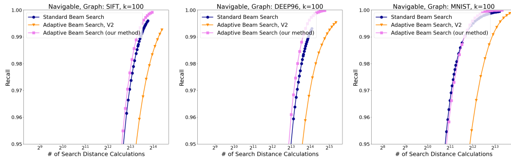
Figure 6: Comparison of generalized beam search termination conditions on navigable graphs across three datasets: SIFT1M, DEEP96, and MNIST (columns), with k = 100 (rows). Adaptive Beam Search consistently outperforms standard beam search, while the alternative Adaptive Beam Search V2 underperforms both by a significant margin.
