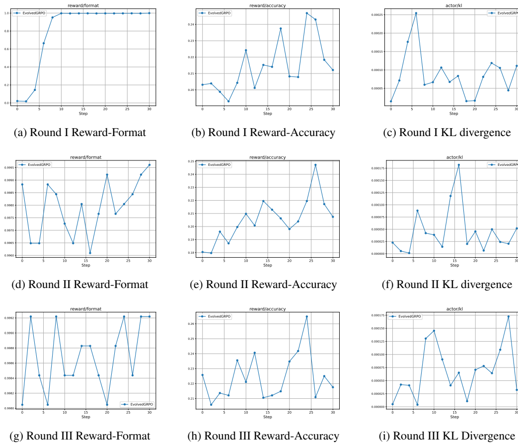
Figure 4: Detailed Evolution Illustration of Reward-Accuracy, Reward-Format, KL Divergence for the answer model over Round I, II, and III.
