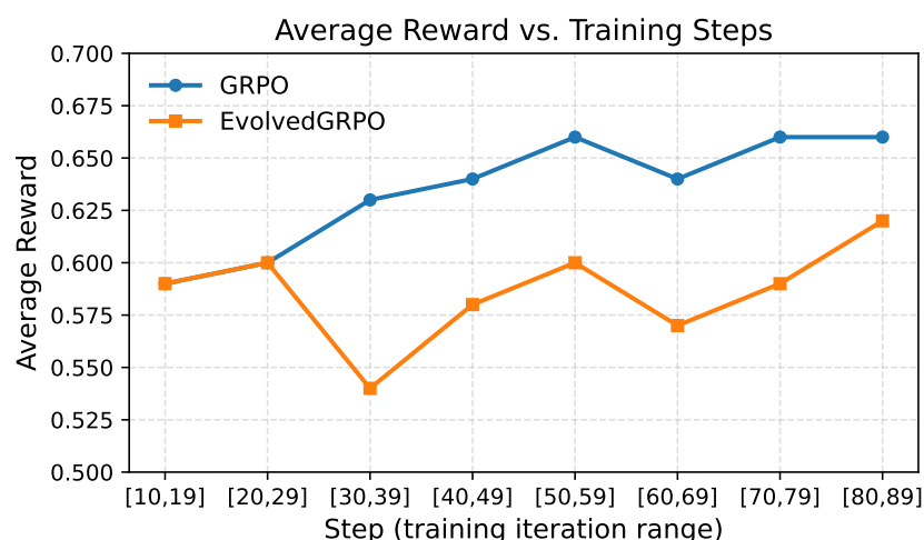
Figure 3: Average reward for the corresponding intervals.
