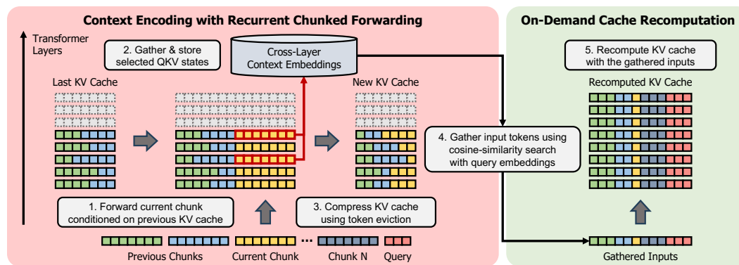
Figure 1: An overview of the proposed framework. REFORM efficiently processes long inputs through two phases. In the recurrent chunked forwarding phase, it segments inputs into chunks and processes them iteratively. In each iteration, REFORM (1) forwards each chunk conditioned on the previous KV cache, (2) extracts key QKV states from selected layers and heads for constructing cross-layer context embeddings, and (3) compresses the cache via token eviction [4]. An early exit strategy skips upper layers beyond those used for embedding collection, further improving efficiency. In the on-demand cache recomputation phase, REFORM selects important tokens via similarity search with the query embeddings (last part of the input), gathers them, and recomputes the KV cache for further generation.
