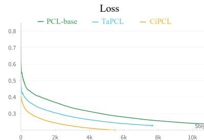
Figure 7: The loss convergence curve on MSCOCO 36 in 29 languages.
