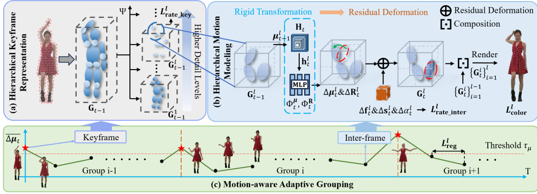
Figure 2: Our 4DGCPro framework. (a) Perceptually-weighted hierarchical 4D Gaussian representation models keyframes at multi-level detail for progressive reconstruction. (b) Hierarchical motion modeling decomposes dynamic scenes into rigid transformations and residual deformations based on the previous frame, while (c) motion-aware adaptive grouping dynamically adjusts to topological changes to enhance temporal consistency and reduce error accumulation. The entire pipeline is end-to-end optimized with layer-wise RD supervision and attribute-specific entropy modeling.
