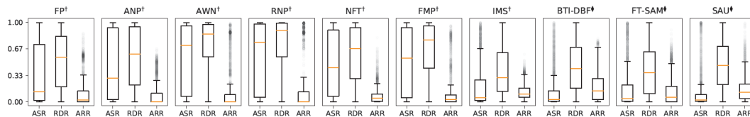
Figure 3: Box plots illustrating ASR, RDR, and ARR results of IMS against various pruning and fine-tuning approaches across all tested settings. †: Pruning, ‡: Fine-tuning.
