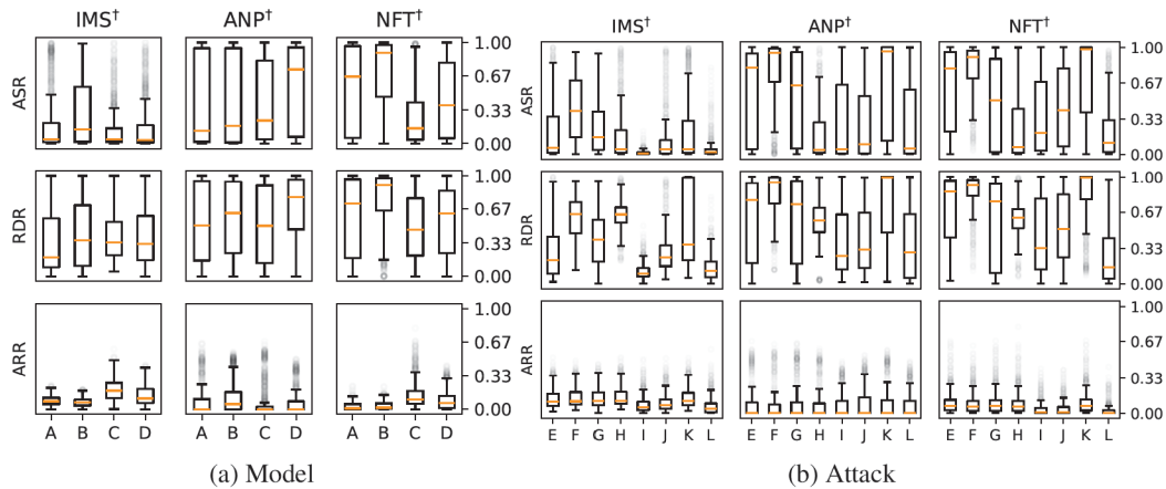
Figure 5: Box plots illustrating ASR, RDR, and ARR results for IMS, ANP, and NFT, across different model and attack settings. In (A) A: VGG, B: ResNet, C: EfficientNet, D: MobileNet. In (B) E: BadNet, F: Blended, G: LF, H: Signal, I: BPP, J: Inputaware, K: SSBA, L: WaNet.
