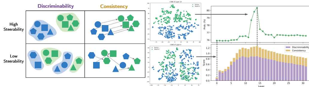
Figure 1: Left: Visualization of discriminability and consistency concepts using contrastive activations. Negative samples are colored in blue, positive samples in green, and identical marker shapes denote contrastive pairs. Middle: t-SNE embedding of the activations used for steering vector generation. Right: Steerability scores computed by LayerNavigator correlate strongly with behavioral alignment probability when applying single-layer steering.
