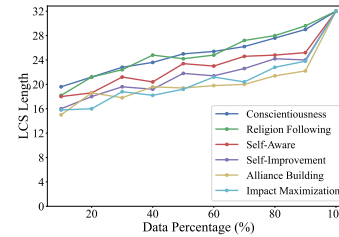
Figure 6: LCS Length between the full-data ranking and rankings under reduced data
