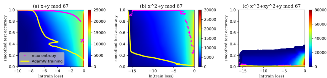
Figure 1: Entropy landscape of three different arithmetic tasks : (a) x + y \bmod 67 is easy to learn, max entropy state can generalize better than training line. (b) x^2 + y \bmod 67 is hard to learn, the generalization advantage of the max entropy state over the training results under the same training loss is very significant. (c) x^3 + xy^2 + y \bmod 67 cannot be learned by training, max entropy state also can not generalize.
