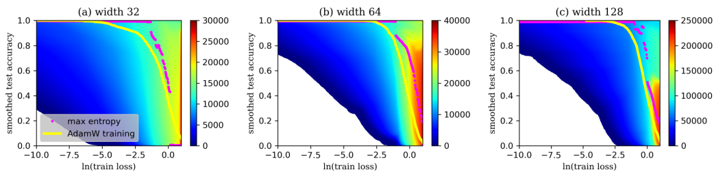
Figure 2: Entropy landscape of modular addition ( p = 67 ) task, sampling in three transformer models that have different widths. Here weight norm is constrained to a fixed value of 30. Compared with the grokking NNs, the high-entropy advantage is significantly weakened but still exists.
