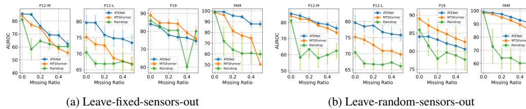
Figure 4: AUROC scores of ATENet, MTSFormer, and Raindrop when dropping variables with various ratios \in [0.1, 0.5] in (a) leave-fixed-sensors-out and (b) leave-random-sensors-out scenarios
