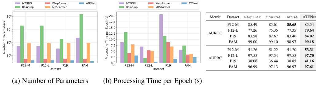
Figure 5: (a) Number of parameters and (b) processing time per epoch for MTGNN, Raindrop, Warpformer, MTSFormer, and ATENet Table 2: Classification performance of ATENet and ablation models
