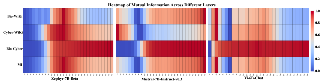
Figure 2: Heatmaps of MI across LLM layers show that lower MI values indicate layers better suited for unlearning, with early layers being more domain-specific and deeper layers more entangled.
