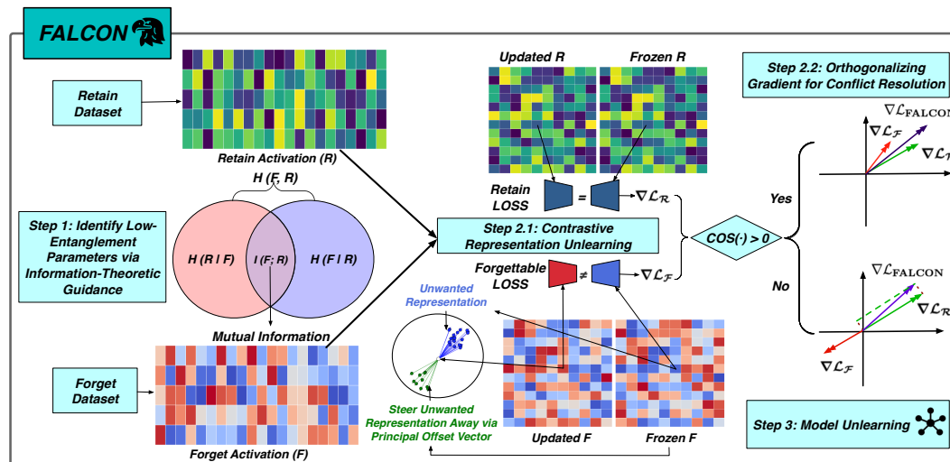
Figure 1: Schematic overview of FALCON. The pipeline comprises three stages: parameter selection based on mutual information (Step 1); contrastive orthogonal unalignment, which consists of contrastive mechanism on both forgetting and retention datasets (Step 2.1) and orthogonal gradient conflict resolution (Step 2.2); and model unlearning guided by these components (Step 3).
