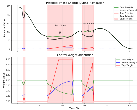
Figure 3: Potential components and control weights during MA-MPPI execution, showing automatic phase transitions in response to detected stagnation (pink regions).
