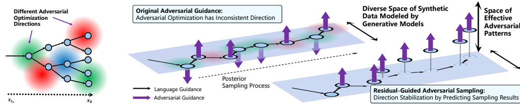
Figure 3: Inconsistent adv. direction problem.
