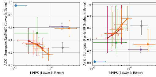
Figure 8: Abstracted label results.
