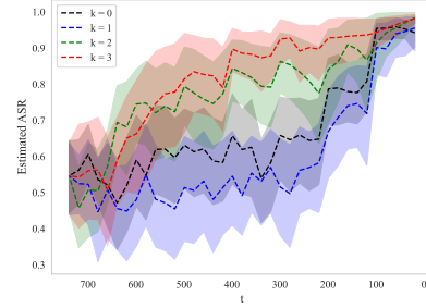
Figure 9: Estimated ASR of \hat{x}_0 after adv. sampling x_t , under different settings of k in Eq. 4. Earlier increase of estimated ASR leads to better naturalness and higher attack transferability.
