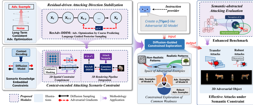
Figure 2: Overview of multi-dimensional instruction uncertainty reduction ( InSUR ) framework.
