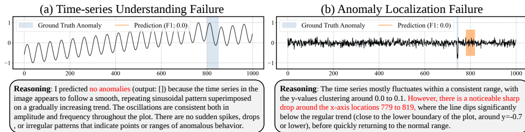
Figure 1: Two representative failure cases of LLM-based TSAD. Although both cases result in an zero F1 score, the reasoning of LLM outputs reveal that the causes stem from different limitations: one in understanding the time series and the other in localization ability.
