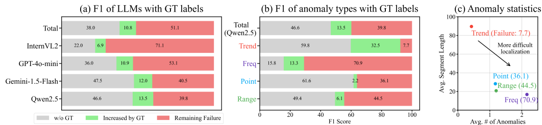
Figure 3: TSAD results with GT anomaly labels to estimate localization failure. (a) shows the F1 improvement by GT labels for each model, (b) shows the improvement by GT labels for each anomaly type, and (c) illustrates the relationship between the number and length of anomalies per type and the remaining failure.
