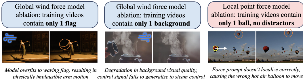
Figure 5: Results from our ablation studies on synthetic dataset design choices. Left: when the global wind force model is trained on a dataset with only one flag, it overfits, causing the woman's arm to wave unnaturally like fabric. Middle: when trained with a single background, the global force model has significantly degraded overall visual quality. Right: when trained without distractor objects, the point force model cannot properly localize motion, applying forces indiscriminately rather than to the intended target.
