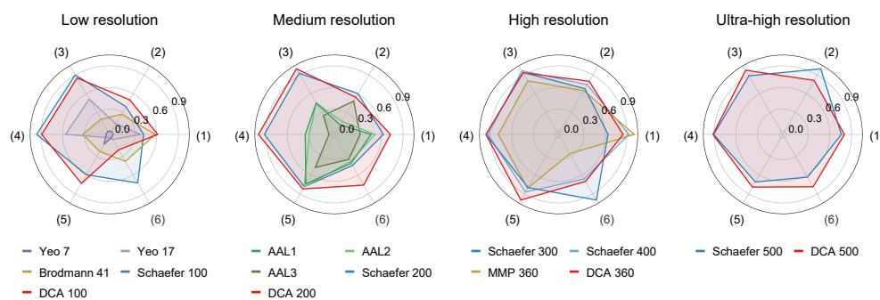
Figure 4: Performance of DCA and baseline atlases across different spatial resolutions on six downstream tasks: (1) gender prediction from resting-state FC (HCP), (2) fluid intelligence prediction from resting-state FC (HCP), (3) classification of 7 cognitive tasks from task-based FC (HCP), (4) classification of 24 cognitive tasks from task-based FC (HCP), (5) ASD vs. control classification from resting-state FC (ABIDE), (6) AD/MCI/CN classification from resting-state FC (ADNI). DCA achieves competitive or superior performance at each resolution level. Values are linearly scaled per task with 0 and 1 corresponding to the lowest and highest performing atlases, respectively.
