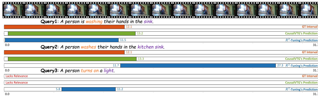
Figure 1: Qualitative examples illustrating two key limitations of existing temporal grounding models. Query1: a successful video grounding example for both VGT models. Query2: a minor rephrasing of the query leads to incorrect localization of R 2 -Tuning due to reliance on superficial co-occurrence cues (e.g., “kitchen”). Query3: the of R 2 -Tuning-Tuning model erroneously predicts a segment for a query describing an unseen action, reflecting its inability to assess query relevance. The proposed CausalVTG, better captures temporal causal structures and abstains when appropriate.
