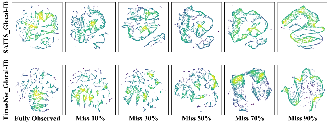
Figure 4: Latent space of SAITS and TimesNet with Glocal-IB on the ETTh1 dataset. Comparison with original models is in the Appendix D.1.
