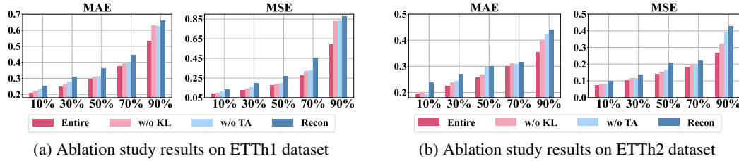
Figure 7: Visualization of ablation study results on ETTh1 dataset. More results are in Appendix D.4.
