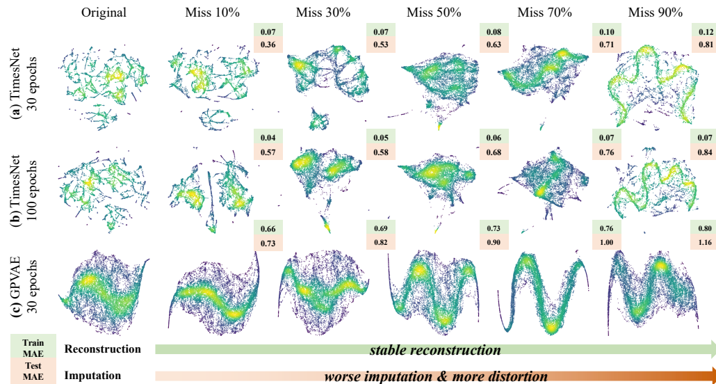
Figure 1: Illustration of optimization dilemma in TSI. We visualize the latent space of two representative models—TimesNet (a-b) and GPVAE (c)—trained under different missing rates and training epochs. Training and test losses are shown in green and orange boxes, respectively.
