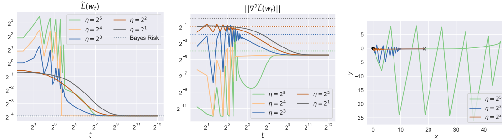
Figure 2: Illustration of large stepsizes accelerating GD. We run constant stepsize GD for an \ell_2 -regularized logistic regression on a two-dimensional separable dataset. The dataset is given by \mathbf{x}_1 = (\gamma, 1) , \mathbf{x}_2 = (\gamma, -2) , y_1 = y_2 = 1 , where \gamma = 0.2 . The regularization is \lambda = 2^{-12} . GD is initialized at \mathbf{w}_0 = 0 . Left: Objective value as a function of training steps. Middle: Sharpness (the largest eigenvalue of the Hessian of the objective) as a function of training steps. Right: GD trajectory in the parameter space, where the black dot is the GD initialization and the black cross is the minimizer. Additional details and plots are given in Appendix E.
