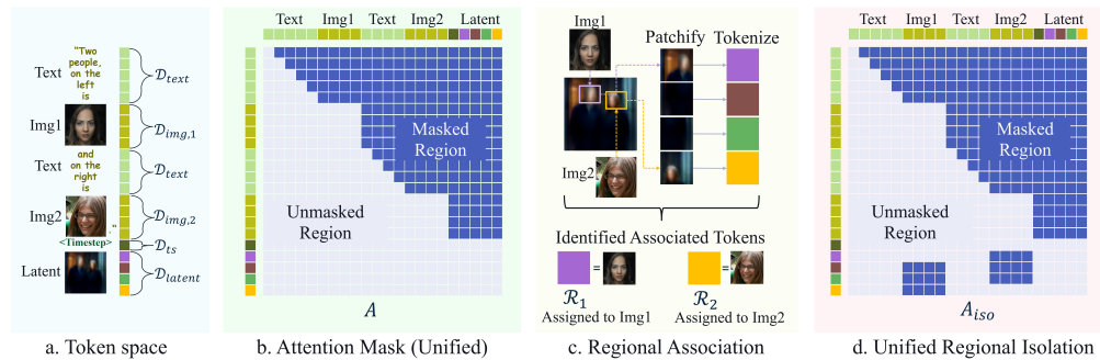
Figure 2: Regional Isolation for Unified Architectures. The updates to the attention mask for regional isolation are illustrated in the differences between Fig.b and Fig.d.
