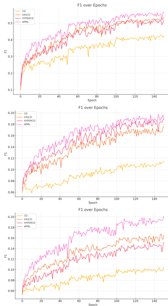
Figure 8: F1 score on the validation set ( Top: PCN. Middle: SN34 Bottom: SN55 ) over 150 epochs for four loss functions: Chamfer Distance (CD), InfoCD, HyperCD, and our proposed APM. The backbone is FoldingNet trained on the PCN dataset.
