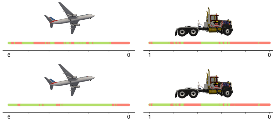
Figure 9: Object detection certification results for Airplane and Truck in GAUSSIANSPLAT scenes. Top row: Certified object detection result. Bottom row: Object detection result obtained via sampling. Green : Certified/Correct Camera Regions. Red : Uncertified/Incorrect Camera Regions.
