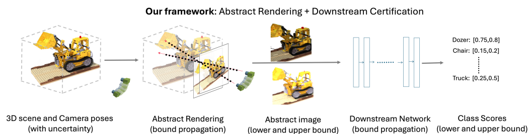
Figure 1: Pipeline of applying abstract rendering to certify downstream network. A range of camera pose uncertainty in a NeRF scene (Left) is propagated step by step through the rendering process (Left Mid) to produce abstract images (Mid). These abstract images are then passed through the downstream network layer by layer (Right Mid), yielding per-class output bounds (Right). For classification, if the lower bound of the Dozer class exceeds the upper bounds of all other classes, the prediction is certified under the given camera uncertainty.
