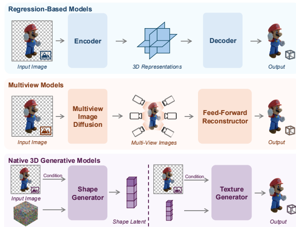
Figure 3: Illustration of the three single-image 3D generation paradigms evaluated in this paper: regression-based methods (OpenLRM [18], SF3D [6]), multi-view approaches (CRM [55], LGM [49], InstantMesh [60]), and native 3D generative models (Trellis [56], Hunyuan3D-2 [64]).
