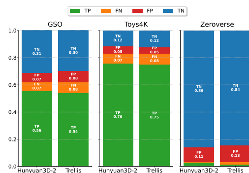
Figure 8: Failure mode of native 3D generative models on meaningless shapes: hallucination of symmetry, shown by the increase of false positives on Zeroverse.
