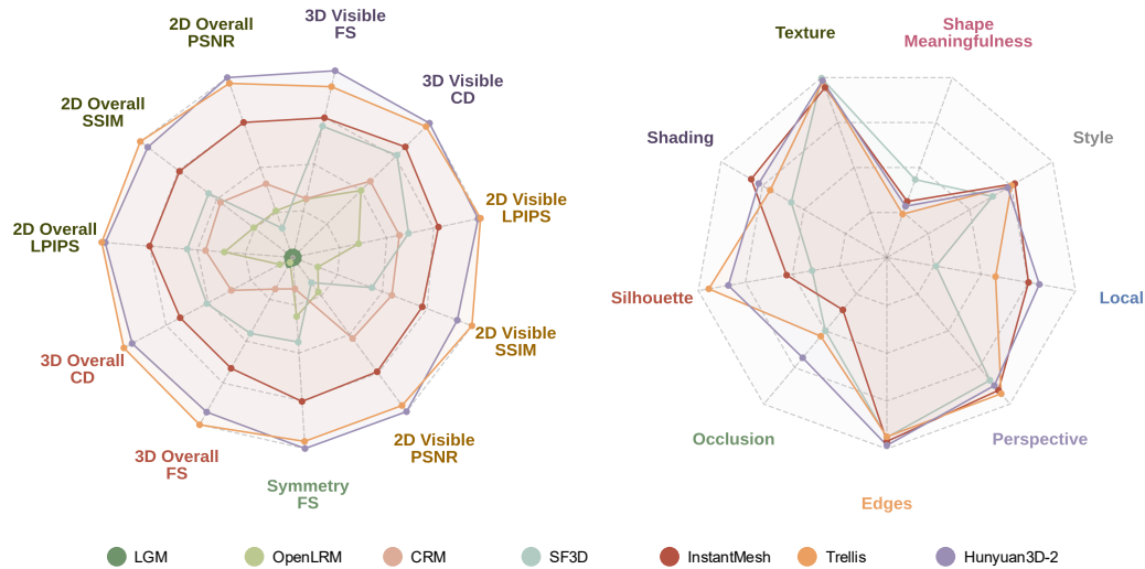
Figure 7: Teaser figure result on the GSO dataset. We observe the same trend as in Toys4K. Left: Our unified evaluation of single-image 3D generation methods. Right: Performance robustness to the perturbation of each cue, lower values indicate higher importance.
