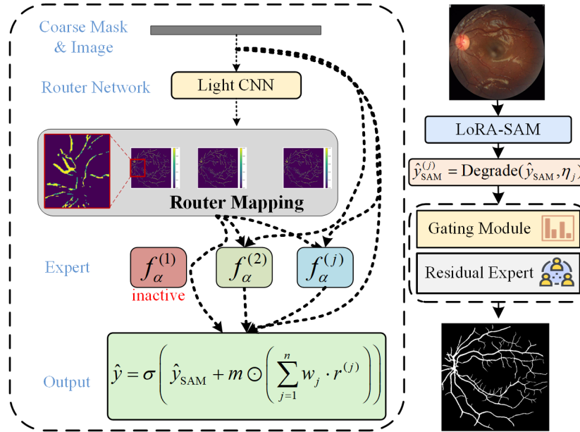
Figure 3: Overview of the FineSAM++ architecture.
