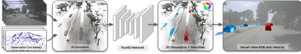
Figure 2: Model overview. Flux4D reconstructs 4D world by predicting 3D Gaussians with velocities given unlabelled sensor observations, and trained with the photometric reconstruction objective. The resultant model can be used for RGB and flow synthesis from novel views.
