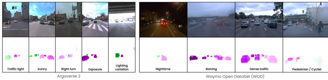
Figure 7: Flux4D reconstruction on Argoverse 2 and WOD.
