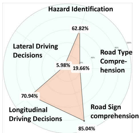
(c) Deepseek-r1
