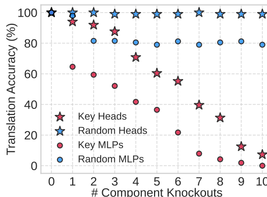
Figure 2: Translation accuracy changes when components are progressively knocked out.
