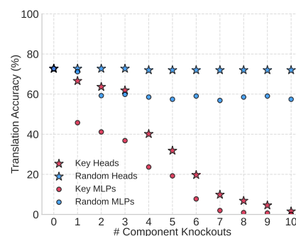
Figure 12: Translation accuracy changes when components are progressively knocked out.
