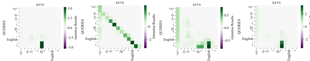
(a) Source Head (18, 17) (b) Positional Head (4, 31) (c) Indicator Head (27, 14) (d) Indicator Head (4, 14)
