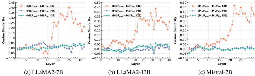
Figure 19: We investigate the projection of each MLP layer ( MLP_{out} - MLP_{in} ) along the direction of the different languages.
