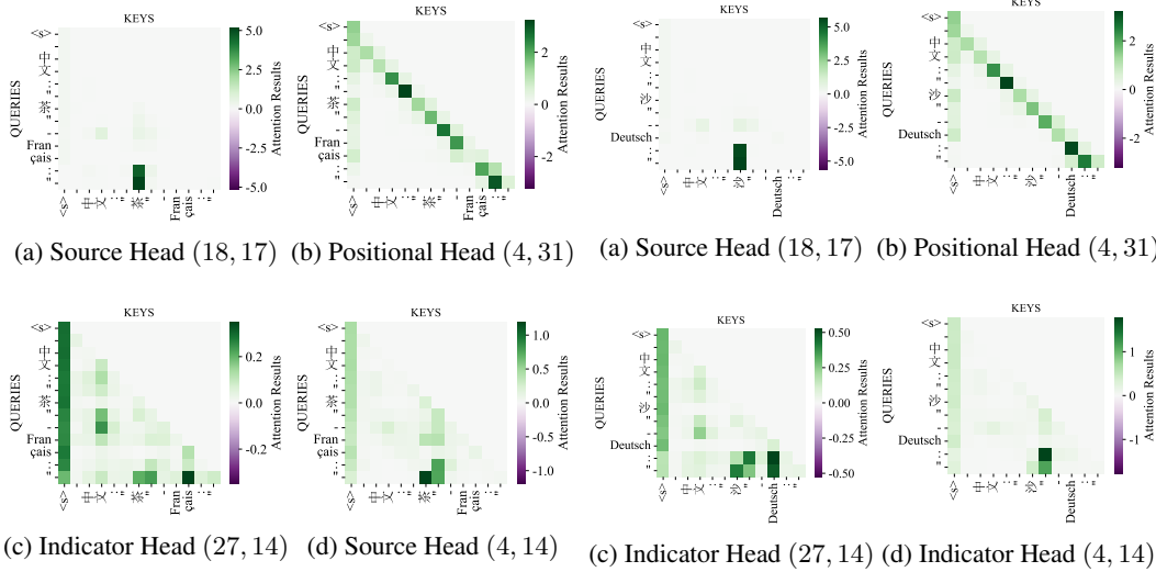
Figure 15: The attention values visualization of the role-classified key heads in Zh \Rightarrow Fr , which show different characteristics of different crucial heads.
