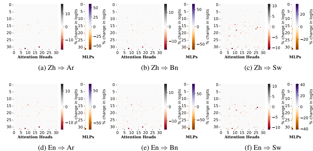
Figure 9: Importance of heads related to translation across different directions. Each square at position (x, y) refers to the x -th head in the y -th layer. Red (Brown) squares denote heads (MLPs) that have a positive impact on predicting the target token, while grey (purple) squares indicate heads (MLPs) with a negative effect.
