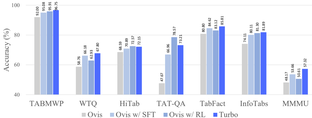
Figure 4: Ablation study of components in TURBO on each dataset. TURBO achieves consistent and significant improvements over the Ovis baseline on all datasets, demonstrating the effectiveness of each introduced component.
