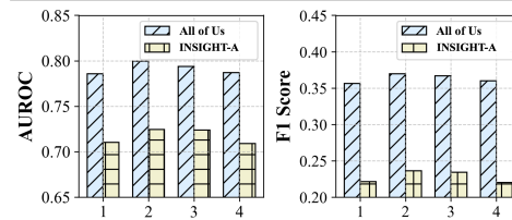
Figure 3: Effect of #aggregation tokens.
