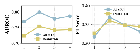
Figure 4: Effect of #transformer layers.
