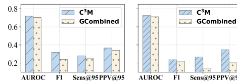
Figure 5: Performance comparison on graph construction strategies.
