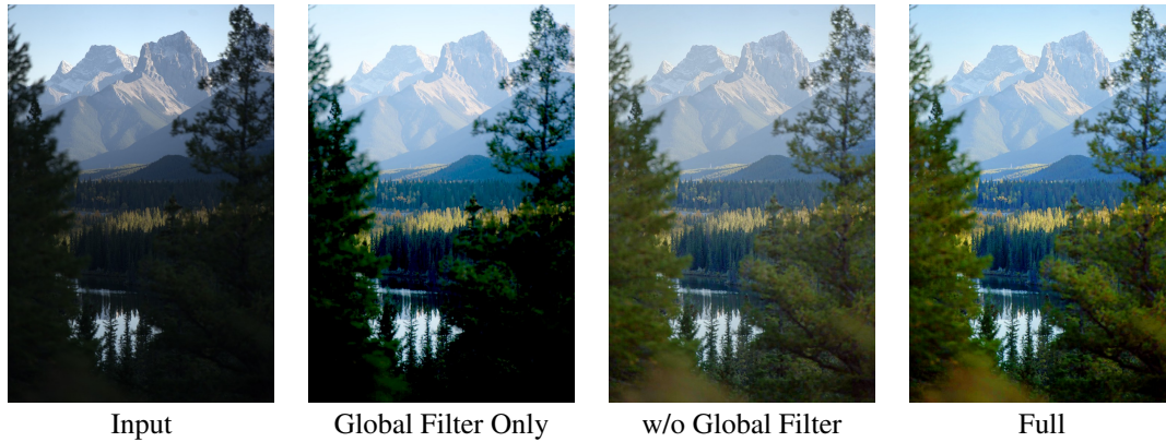
Figure 20: Visual comparison of different module configurations. The Global Filter alone provides basic adjustments but lacks expressiveness and cannot achieve high brightness levels. Without the Global Filter, the image shows improved color but insufficient contrast. The full model combines the strengths of all components, delivering optimal brightness, contrast, and color expressiveness for the most visually appealing result.
