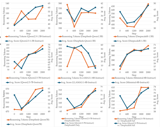
Figure 3: The averaged number of reasoning tokens and scores over steps (best viewed magnified).
