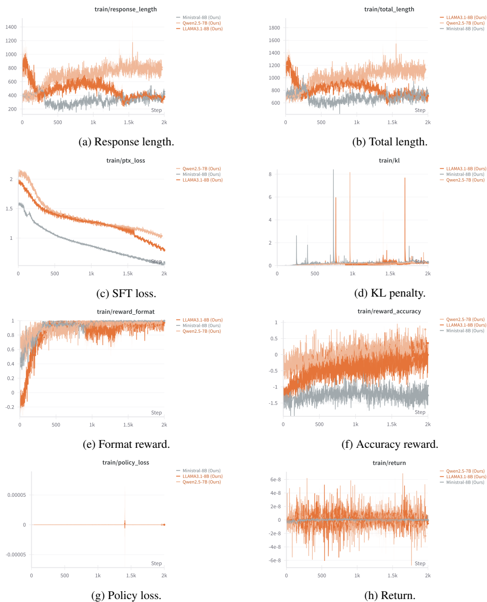
Figure 35: Training dynamics across model families: Qwen2.5-7B, LLaMA3.1-8B, and Ministral-8B (best viewed magnified).
