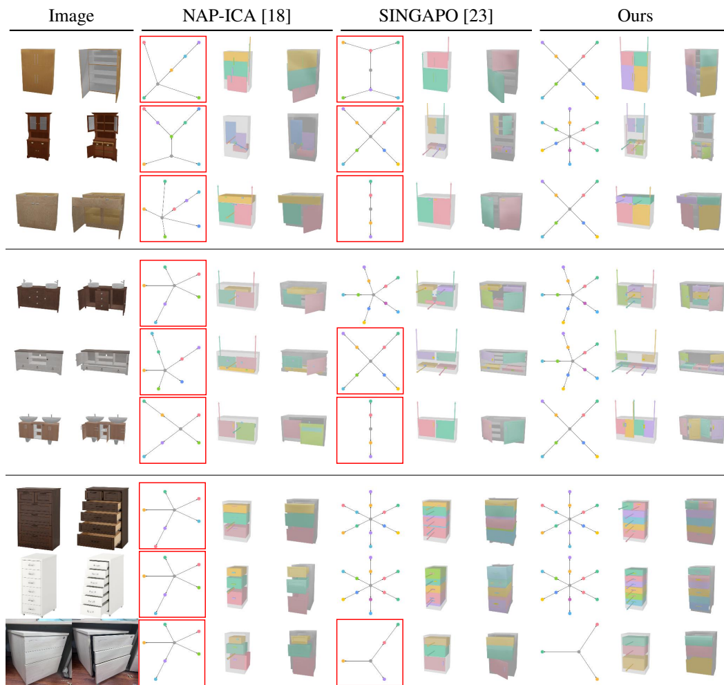
Figure 5: Visual comparison between the proposed DIPO and two baselines. The first two columns show the dual-state image pairs. The prediction results of articulate graph, the part layout and joint visualization in resting state, and the final geometry in articulated state are also illustrated. The first three rows are sampled from the PM dataset, the middle three rows are from the ACD dataset, and the last three rows are real-world images. Incorrect parts connections are marked with red box.
