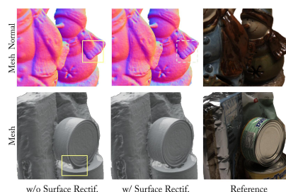
Figure 7: Qualitative Studies for the Surface Rectification. Facilitation for sharp and accurate surfaces is made.
