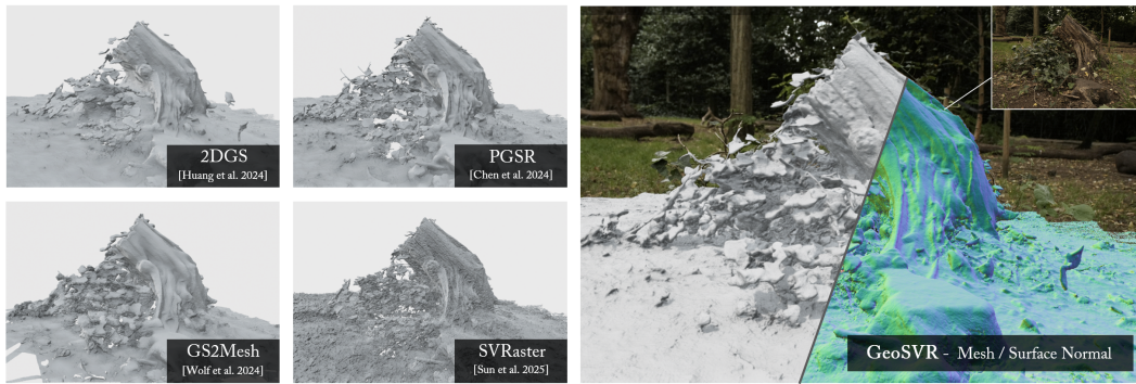
Figure 1: Geometric Sparse-Voxel Reconstruction. Our method, abbreviated as GeoSVR, delivers high-quality surface reconstruction for intricate real-world scenes based on explicit sparse voxels. Our superiority is exhibited compared to the state-of-the-art approaches built upon Gaussian Splatting, which encounter rough, inaccurate, or incomplete recovery problems even with help from external estimators, excelling in delicate details capturing with high completeness and top-tier efficiency.
